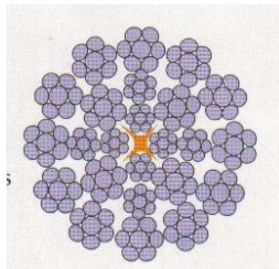
24X7 DYFORMED GALVANIZED
