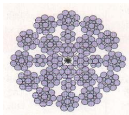
24X17 DYFORMED GALVANIZED
